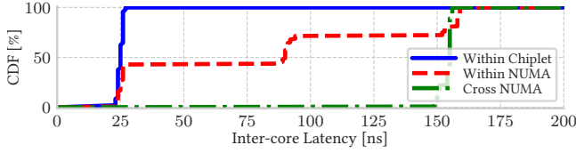
Fig. 3: Cumulative distribution function (CDF) of core-to-core latency in AMD EPYC Milan CPUs
