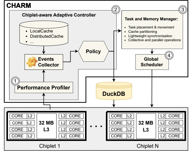
Fig. 6: CHARM architecture
