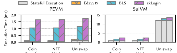
Figure 2: Execution breakdown of common smart contracts.
