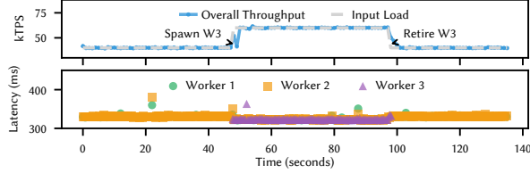
Figure 9: Elastic scaling for load fluctuations.
