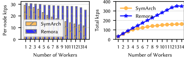
Figure 4: Comparison with other work using symmetric architecture.
