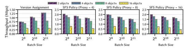
Figure 12: VerAssign. and Sched. (SFS) module sensitivity analysis.
