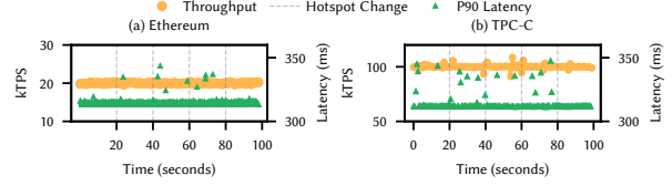
Figure 10: Dynamic hotspot workloads.
