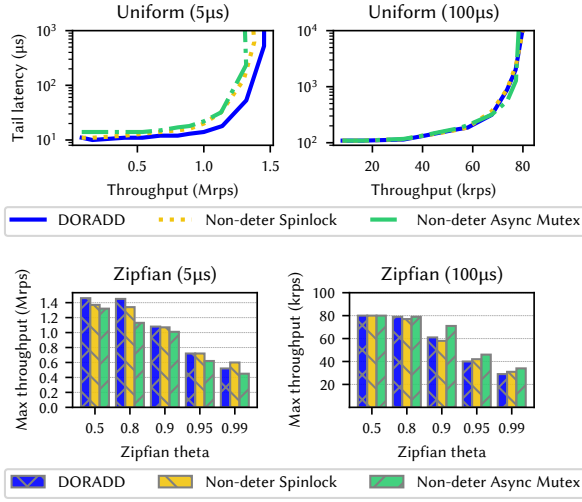
Figure 7. Performance comparison with non-deterministic systems.
