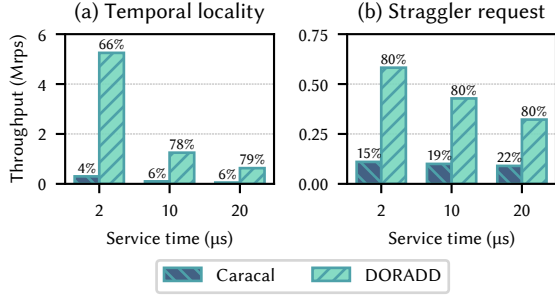
Figure 2. Caracal and DORADD throughput in synthetic read-spin-write workloads. The percentage denotes the ratio of actual throughput to the ideal throughput.
