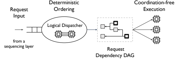
Figure 3. DORADD Architecture. The cores are split into dispatcher and worker cores. The pipelined dispatcher cores construct a dependency DAG of requests, while worker cores execute them in a coordination-free manner.
